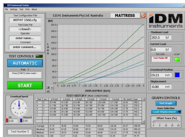
Foam Compression Tester sample test screen
